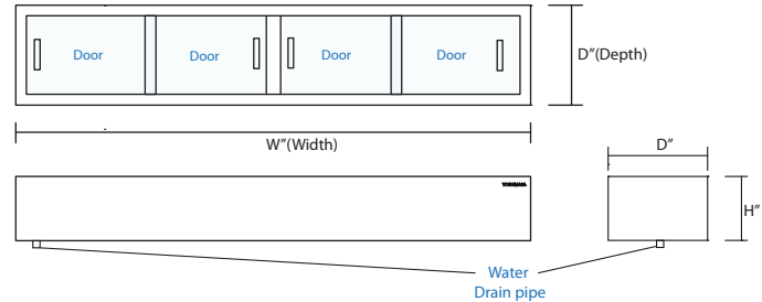
Remote Type Sushi Display Case
