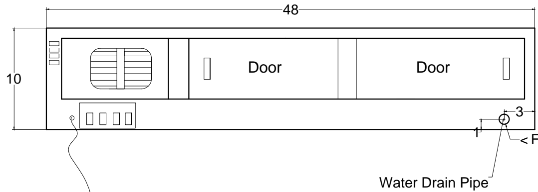
Rear view
